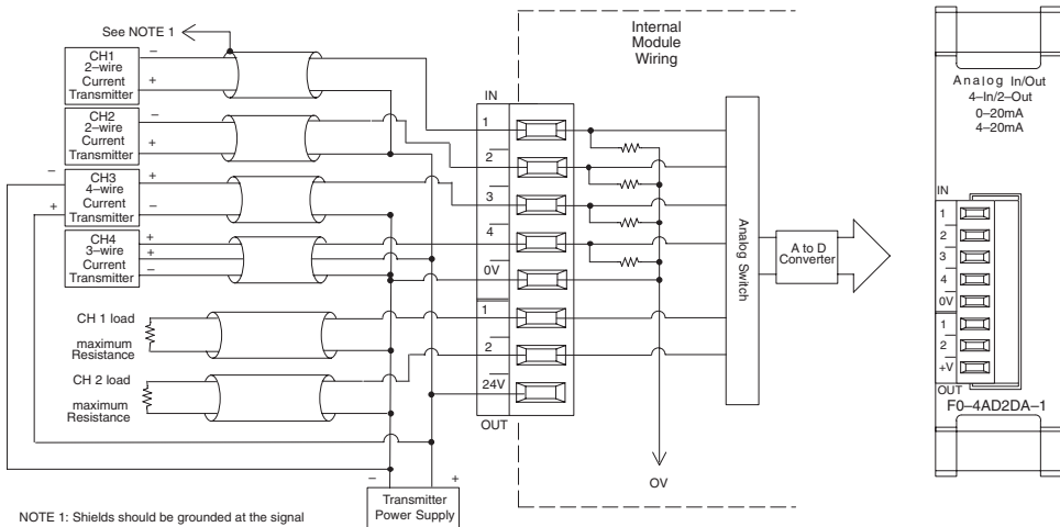
Typical User Wiring
