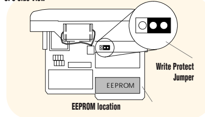
CPU Side View
